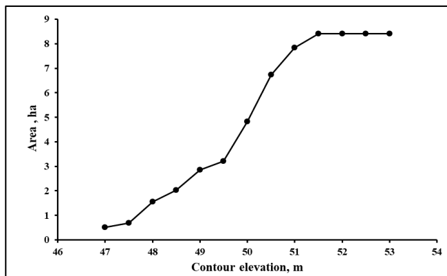
Fig 4: Relationship between contour elevation and waterlogged area for Jhilli-B
