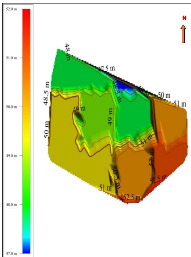
Fig 1: Contour Map of Harpur Jhilli Chaur area - A
