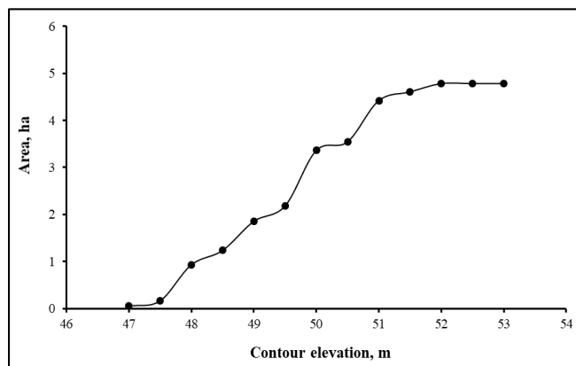
Fig 3: Relationship between contour elevation and waterlogged area for Jhilli -A
