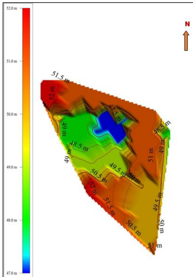
Fig 2: Contour Map of Harpur Jhilli Chaur area - B
